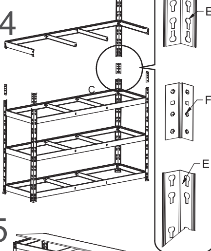
DETAIL E
