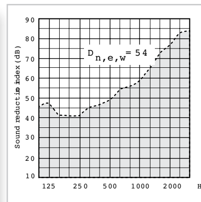
Fresh 80-dB with 400mm wall pipe.
