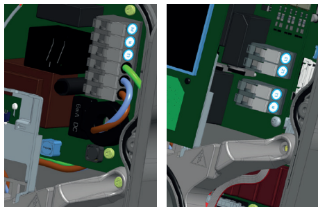
Figure 7a and 7b: Attaching individual charging cable wires on the Pro-line and S-line models.
