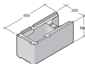
Betonivaluharkko BVH-200 kulma
