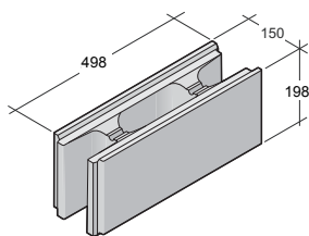
Betonivaluharkko BVH-150
