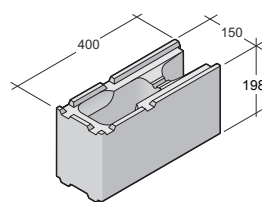
Betonivaluharkko BVH-150 kulma
