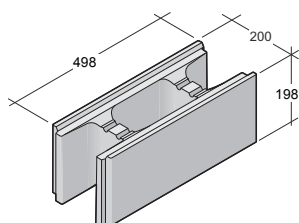
Betonivaluharkko BVH-200
