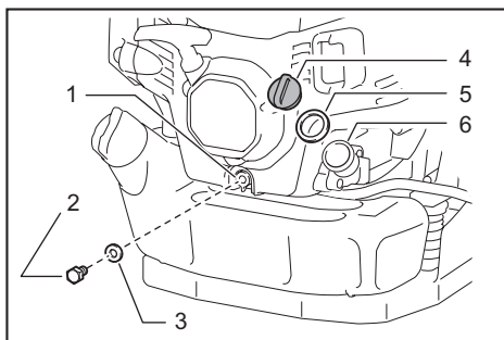
► 1. Drainage hole 2. Oil drain bolt 3. Gasket (aluminum washer) 4. Oil cap 5. Oil cap gasket 6. Oil port
