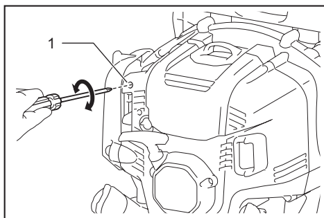
► 1. Idling adjusting screw
