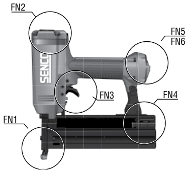
Finish Nailer
