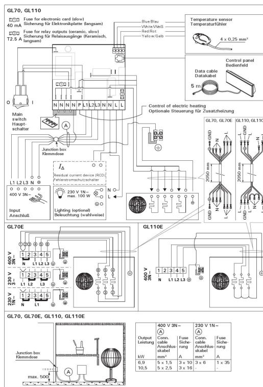
Electrical connections
