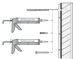
Concrete/Solid construction
