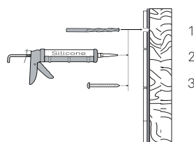
Wood/Sheet construction
