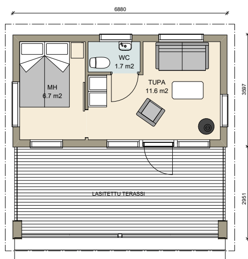
tupa, 1 mh, wc
