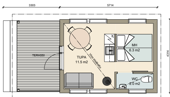
tupa, 1 mh, wc
