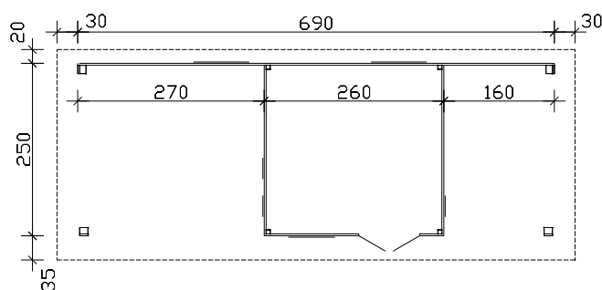
Floor plan, cross-section and elevations M 1: 100
