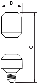
TForce LED EU SON-T 70W 50khrs 4000K
