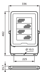
BVP165 LED210/840 PSU 200W AWB CE
