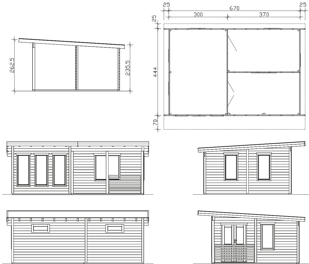
Floor plan, cross-section and elevations M 1:100
