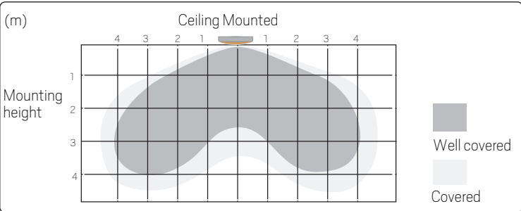
Range - Ceiling mounting pattern (Unit: m) Suggested installation height: 2.5-4m
