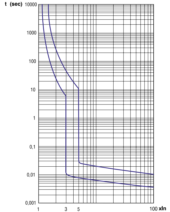
MDC 60 - 100 Characteristic B
