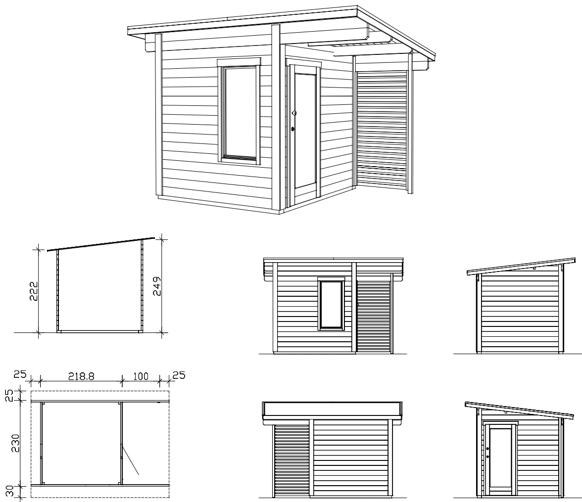
Floor plan, cross-section and elevations M 1:100
