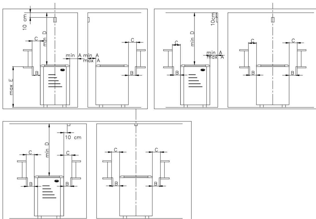
Figur 2. Sensordosans installation
