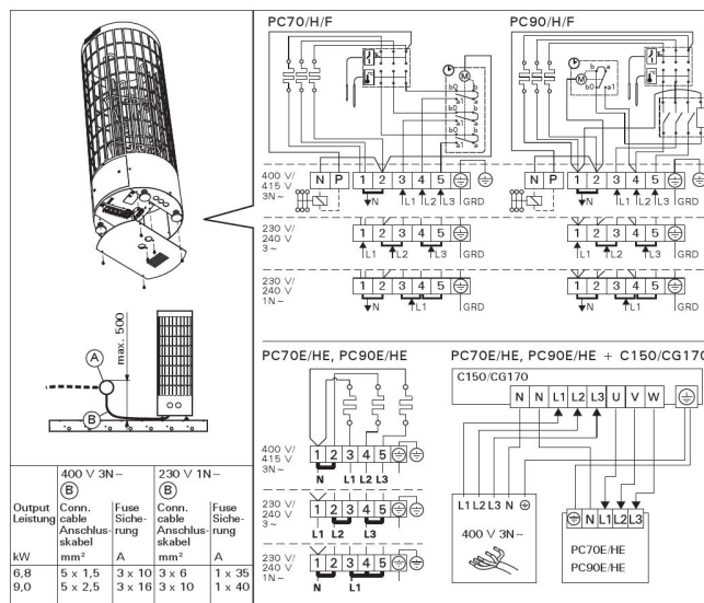
Electrical connections
