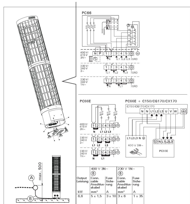
Electrical connections
