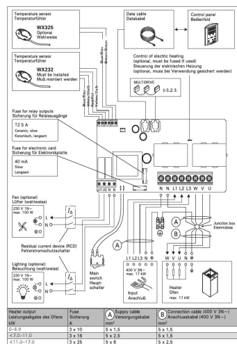
Electrical connections of control unit C6170 and HL heater
