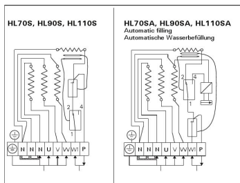
Electrical connections
