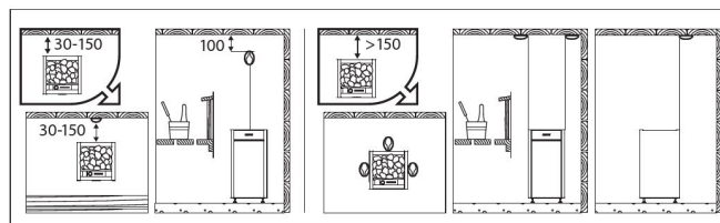
Installing the temperature sensor (all dimensions in millimeters)
