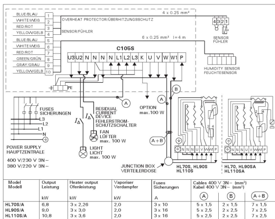
Electrical connections of control unit C105S and HL5(A) heater
