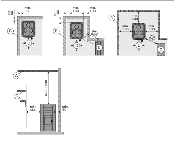
Safety distances (all dimensions in millimeters)
