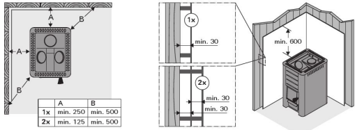
Protective covers (all dimensions in millimeters)
