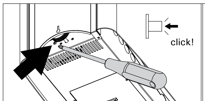
Figure 12. Resetting the overheat protector
