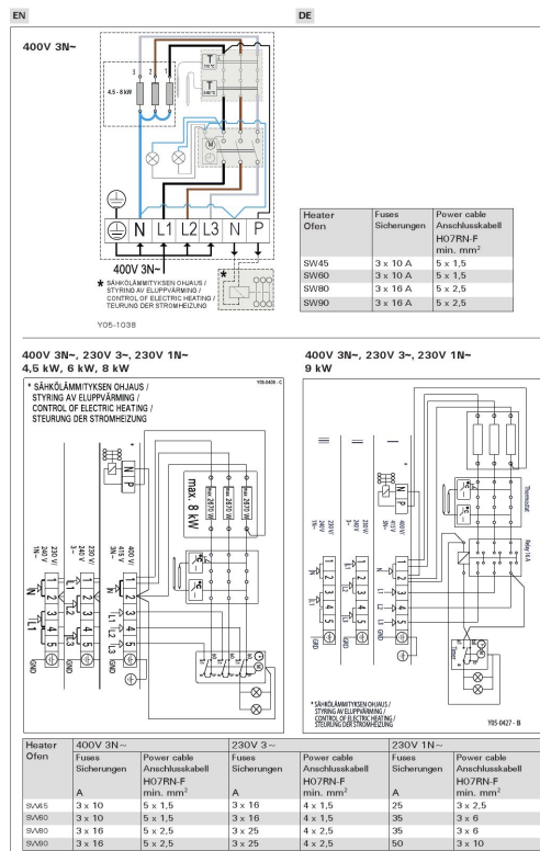
Figure 11a. Electrical connections (SW45, SW60, SW80, SW90)
