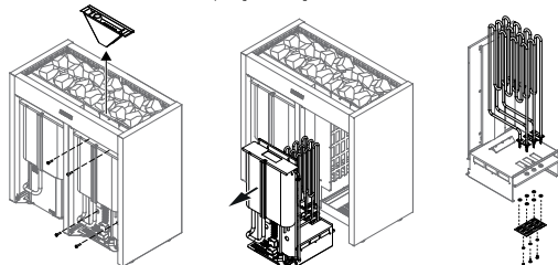
Replacing the Heating Elements
