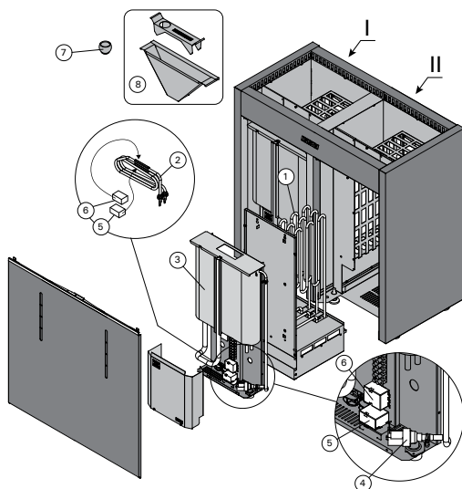
Replacing the Heating Elements
