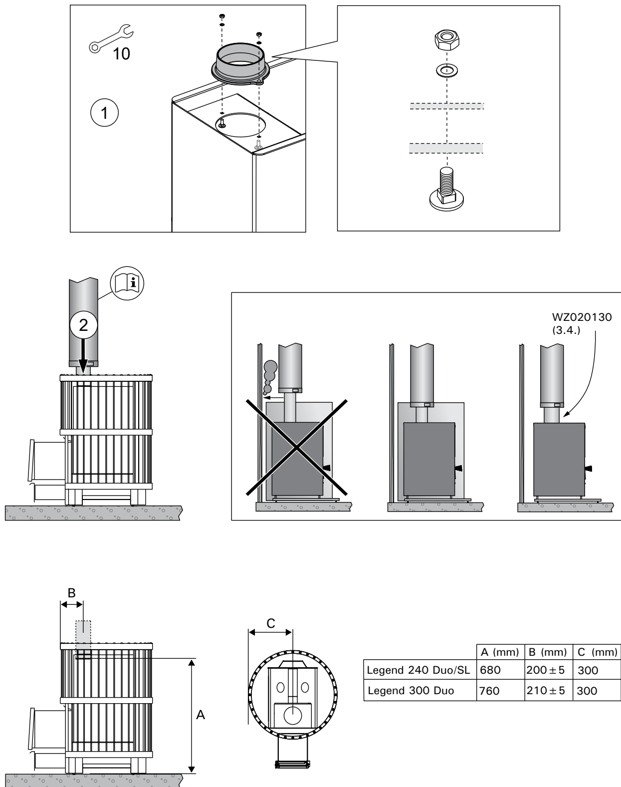
Kuva 11. Connecting the Stove to a Harvia Steel Chimney
