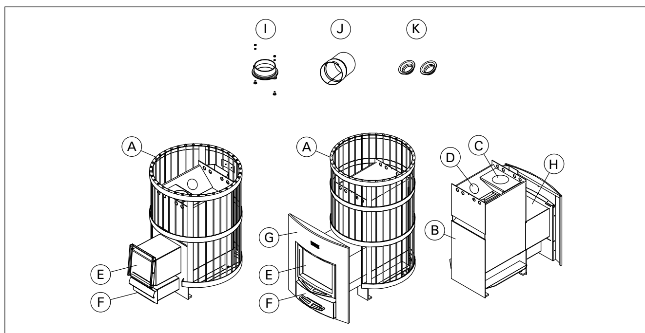
Figure 1. Stove parts. Note! Unauthorised modification of the stove is prohibited.
