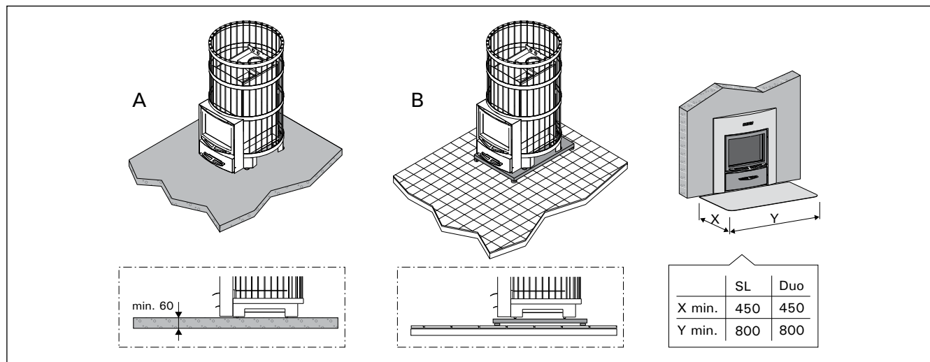
Figure 8. Protecting the floor (all dimensions in millimeters) Abbildung 8. Bodenschutz (alle Abmessungen in Millimetern)
