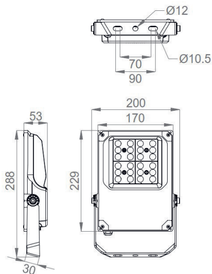
Onnline valonheitin Onnflood Multi IP65 2800-7500LM 50W
