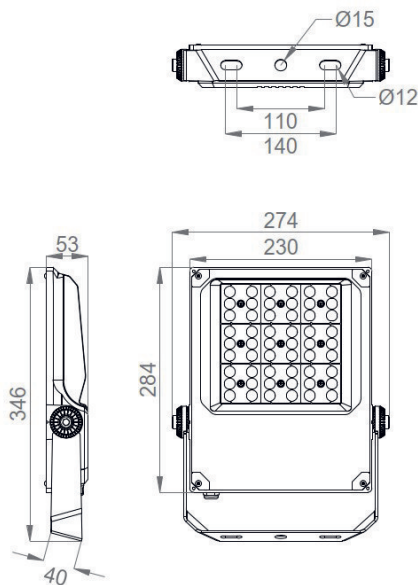
Onnline valonheitin Onnflood Multi IP65 7000-14250LM 100W 3CCT
