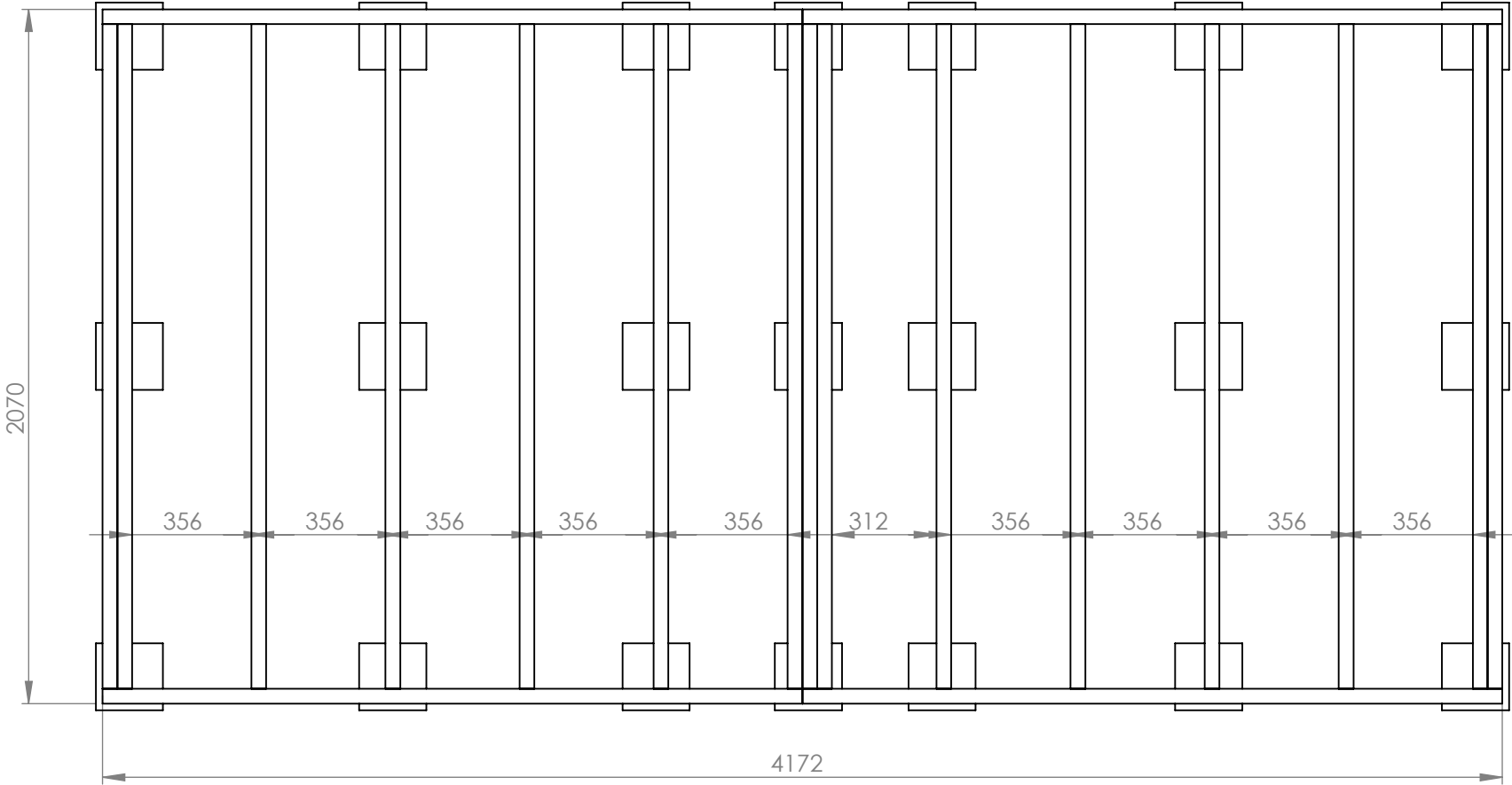
Base frame and recommended support positions
