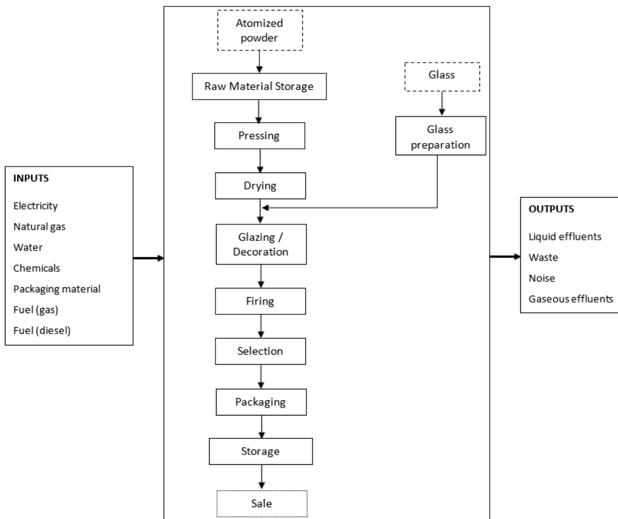
Figure 1 – Flowchart of the manufacturing production process.
