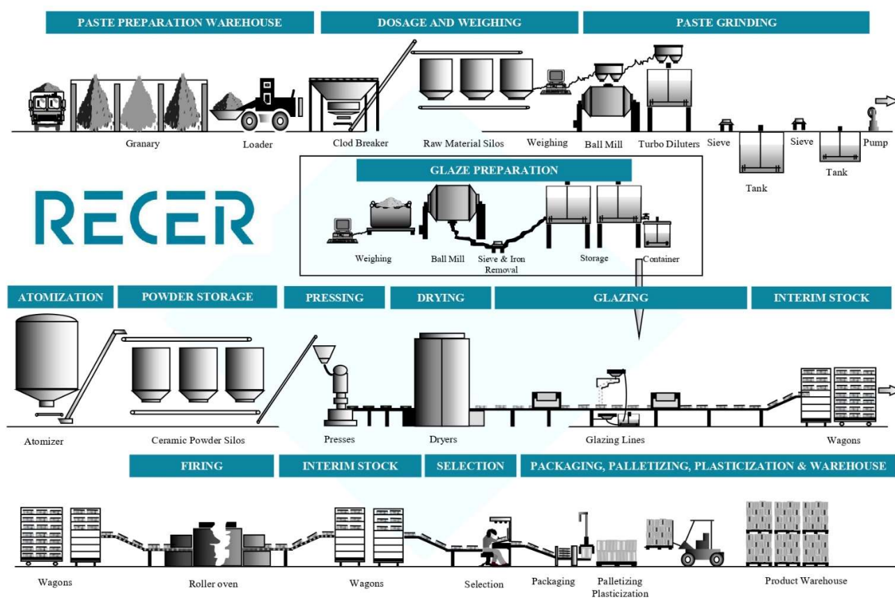
Figure 2 - Production process
